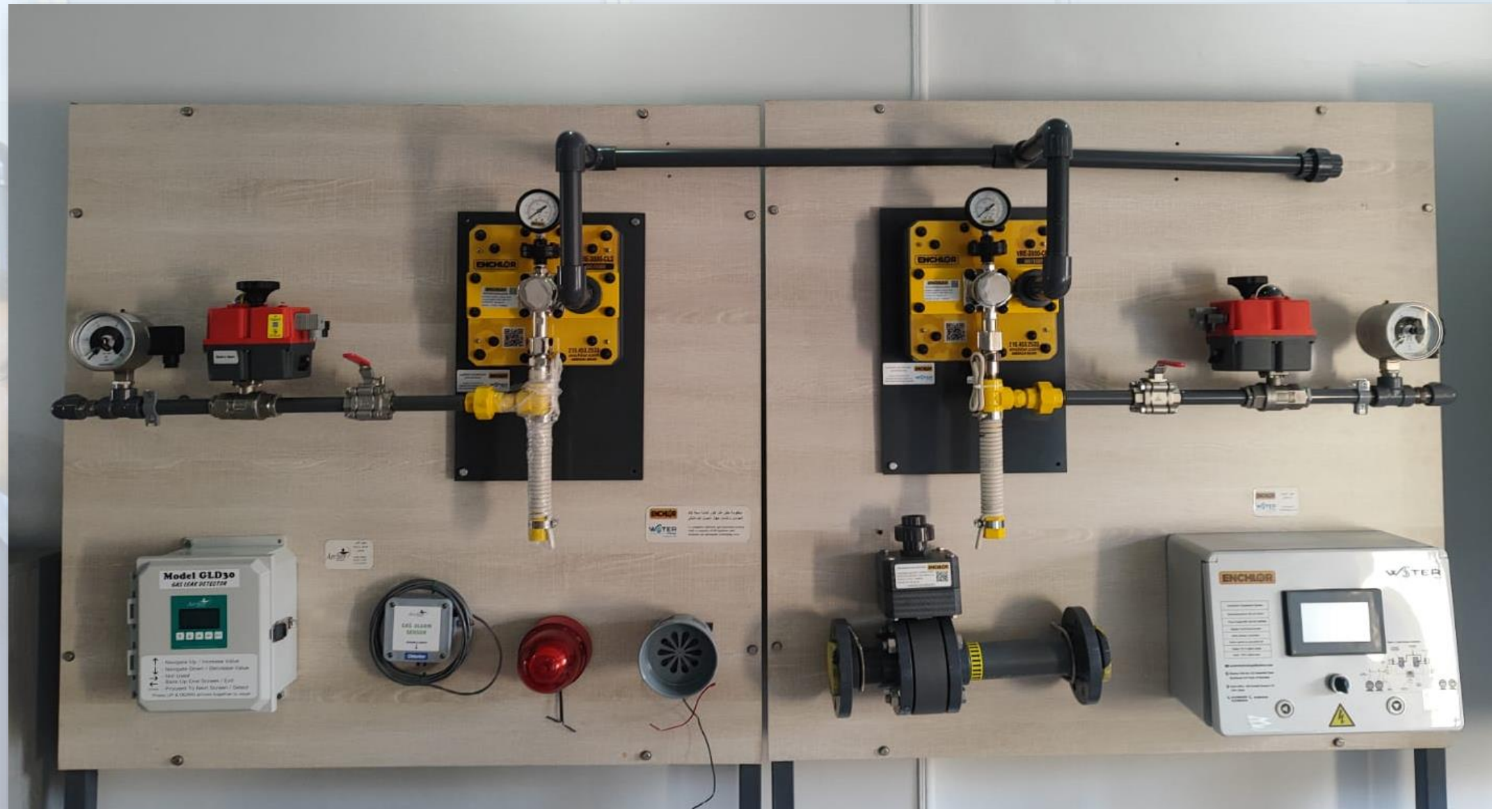
Automatic switchover system with a capacity of 40 kg/h + alarm system and its components
